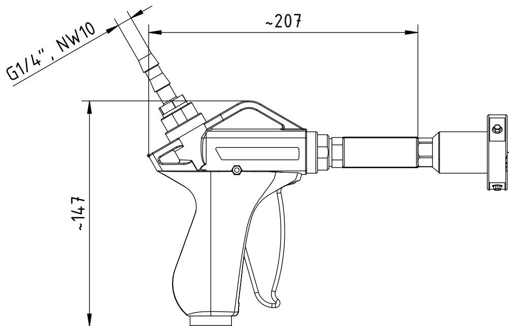
Fig. 17: Dimensions PR36/OE ion blower pistol
