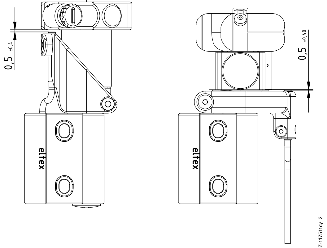
Fig. 9: Speed monitoring
