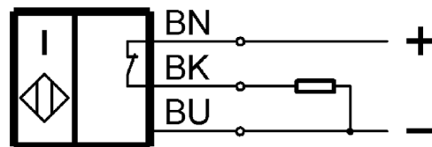
Fig. 10: Speed monitoring Circuit diagram
