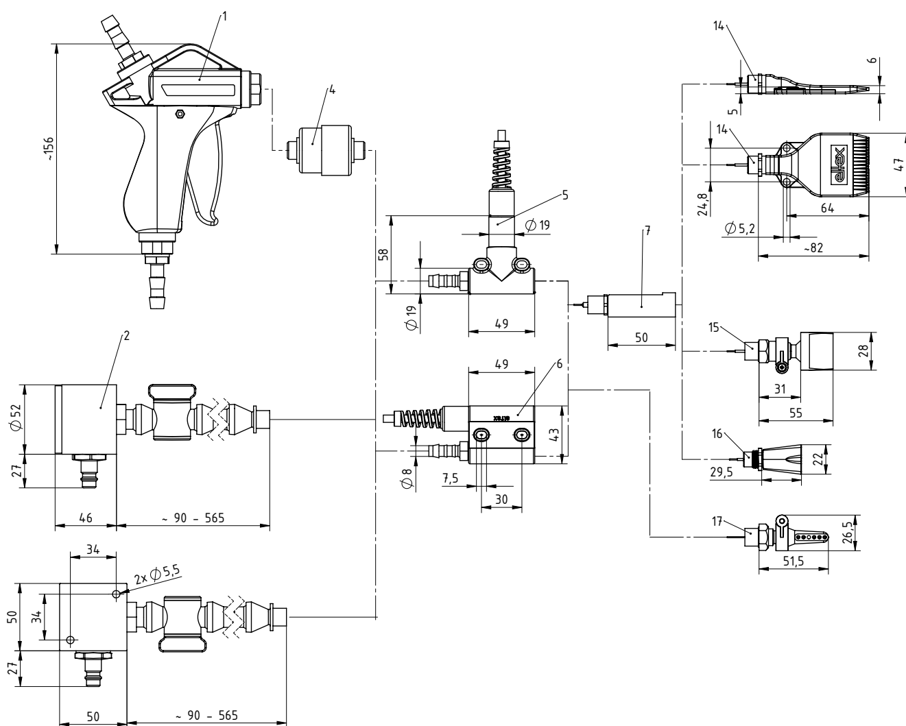
Fig. 12: Drawing -No. Z-116969ey_2 Dimensions ion blower pistol, various nozzles and accessories
