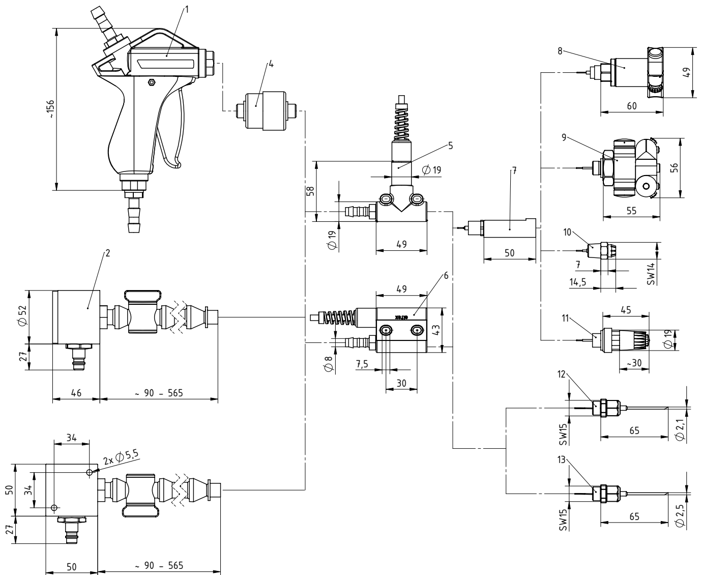
Fig. 11: Drawing -No. Z-116969ey_1 Dimensions ion blower pistol, various nozzles and accessories
