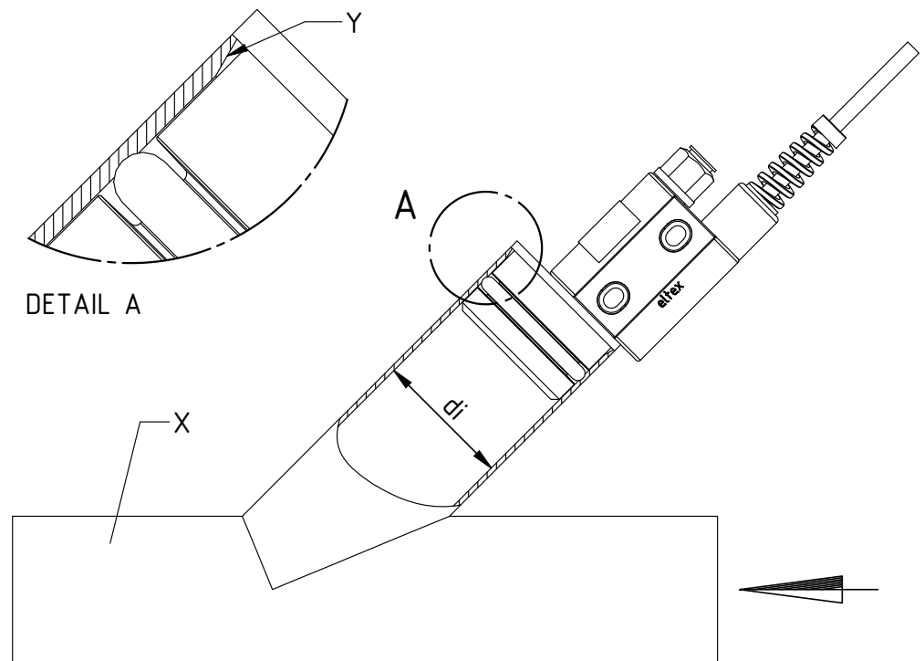
Fig. 5: Installation situation Example: EAR36E/AKS_ _L
