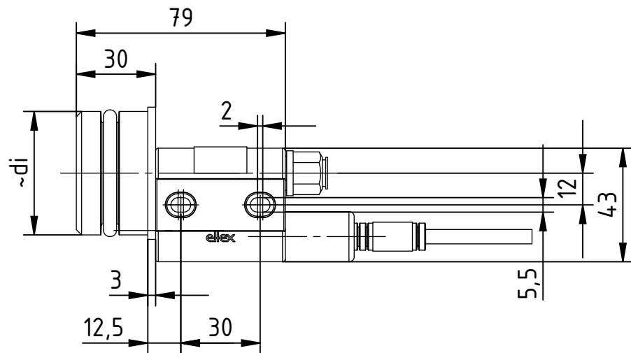
Fig. 18: Dimensions EAR36E/A discharge adapter axial
