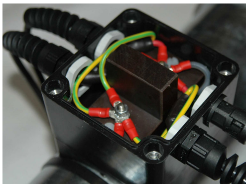
Fig. 3: High voltage distributor with screw-type contacts
