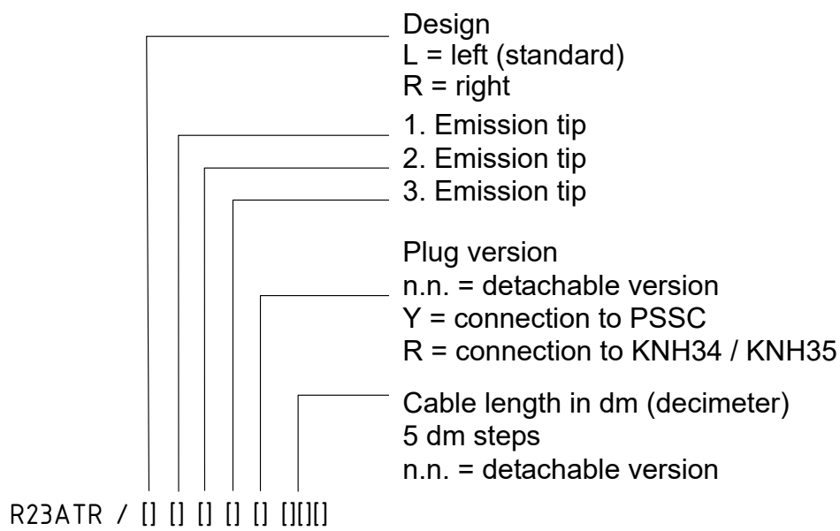
Fig. 5: R23ATR point charging bar
