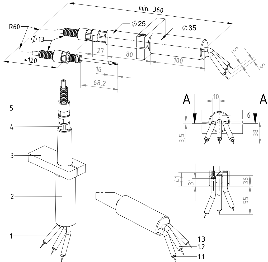
Fig. 1: R23ATR/LAAA point charging bar design left with emission tip Type A
