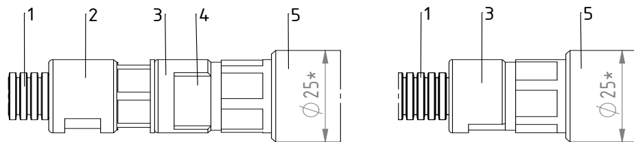
Fig. 12: R23ATR male connector of the high voltage cable
