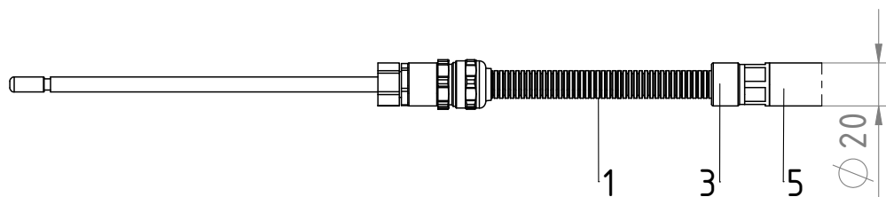
Fig. 8: R23ATR11 point charging bar with fixed high voltage cable, plug version Y, X
