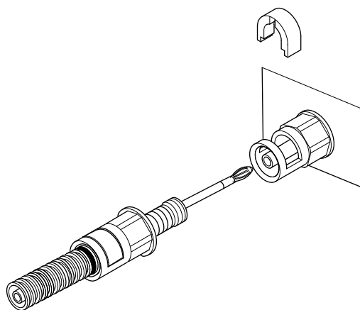
Fig. 13: Connecting the high voltage cable
