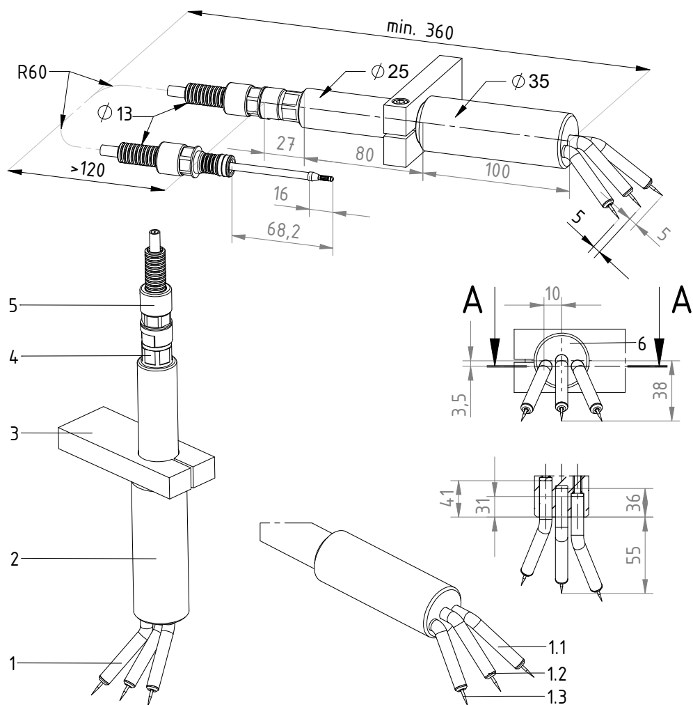
Fig. 2: R23ATR/RAAA point charging bar design right with emission tip Type A
