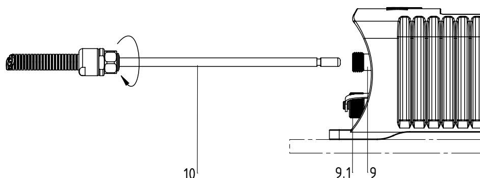
Fig. 15: Connecting the high voltage cable
