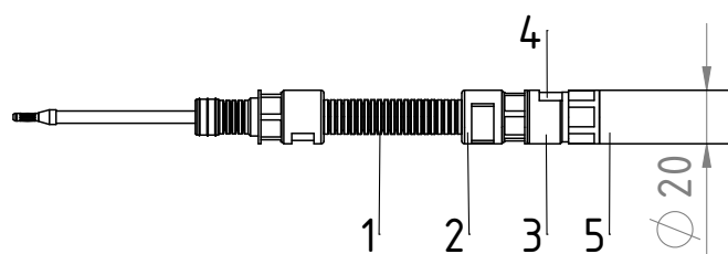
Fig. 10: R23ATR11 point charging bar with detachable high voltage cable, plug version R, U
