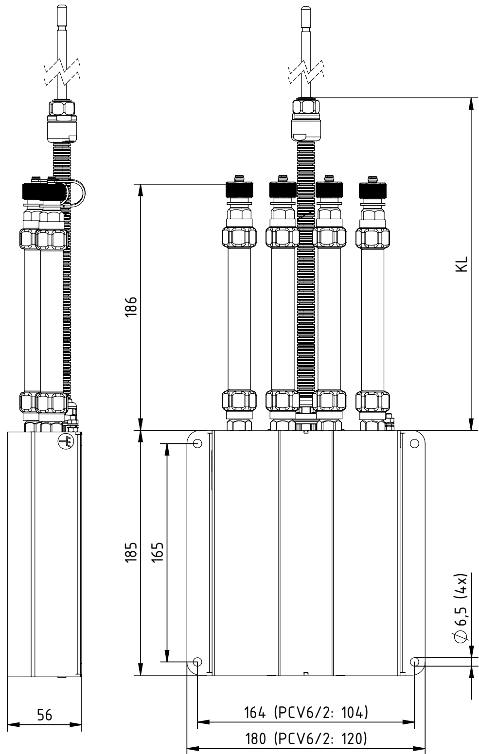
Fig. 7: Dimensions Distributor PCV6/2, PCV6/4
