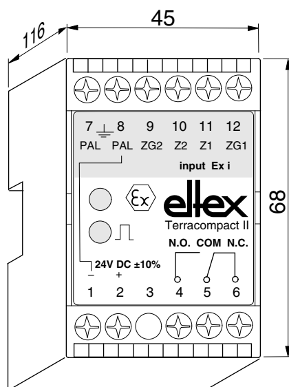
Fig. 8: Terracompact II TCO030 with ter- minal assignment
