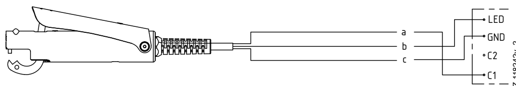
Fig. 12: Connection example of the ground contactors TERRA-L with integrated status LED
