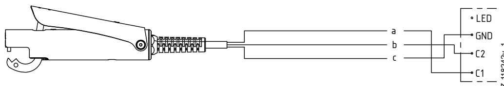
Fig. 11: Connection example of the ground contactors TERRA-L
