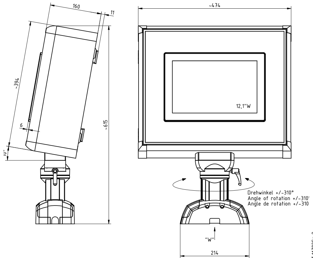
Fig. 49: Dimensions, Remote control ECC/GH and ECC/GI
