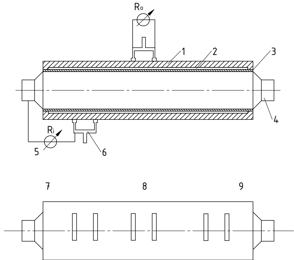
Fig. 15: Measuring set-up
