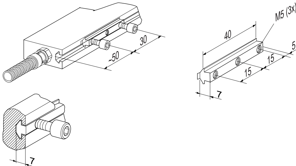
Fig 11: Assembling with sliding nuts
