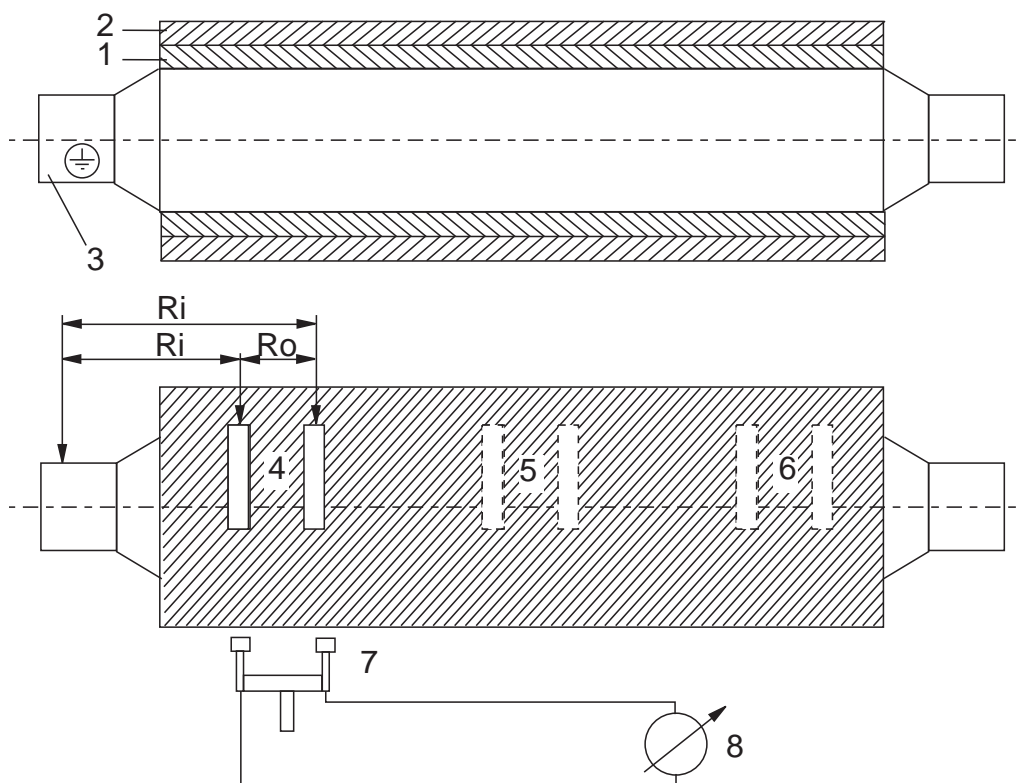
Fig 14: Measuring set-up
