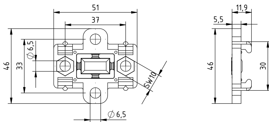
Fig. 13: Support standard
